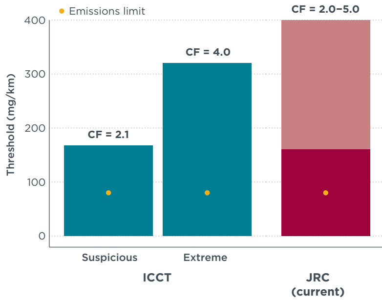
Figure 5. ICCT recommended thresholds for Categories 3 and 4 compared to the existing Category 3 threshold. The 2021 proposed JRC threshold is based on a relative analysis and therefore is not shown as it is defined based on results from other vehicles.
