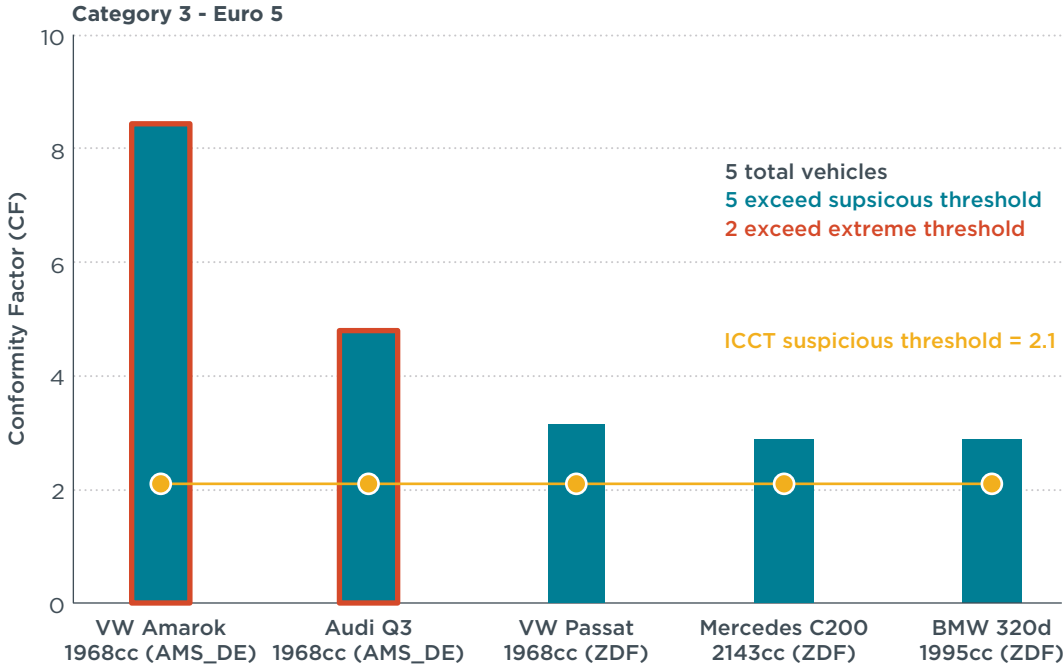
Figure 12. Average NO x conformity factors for independent Category 3 tests by Euro 5 diesel vehicle model, showing only those with averages exceeding the suspicious threshold. The test source is indicated in parenthesis. The red outline indicates that the vehicle model's average emissions exceed the extreme threshold (CF = 4.0).
