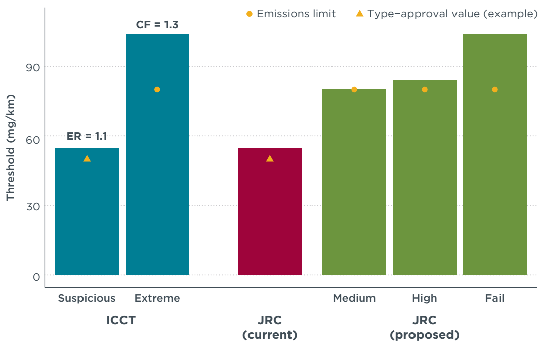
Figure 3. ICCT recommended thresholds compared to existing and proposed thresholds for Category 1 tests, using an example of a Euro 6 vehicle type-approved at 50 mg NO x /km.
