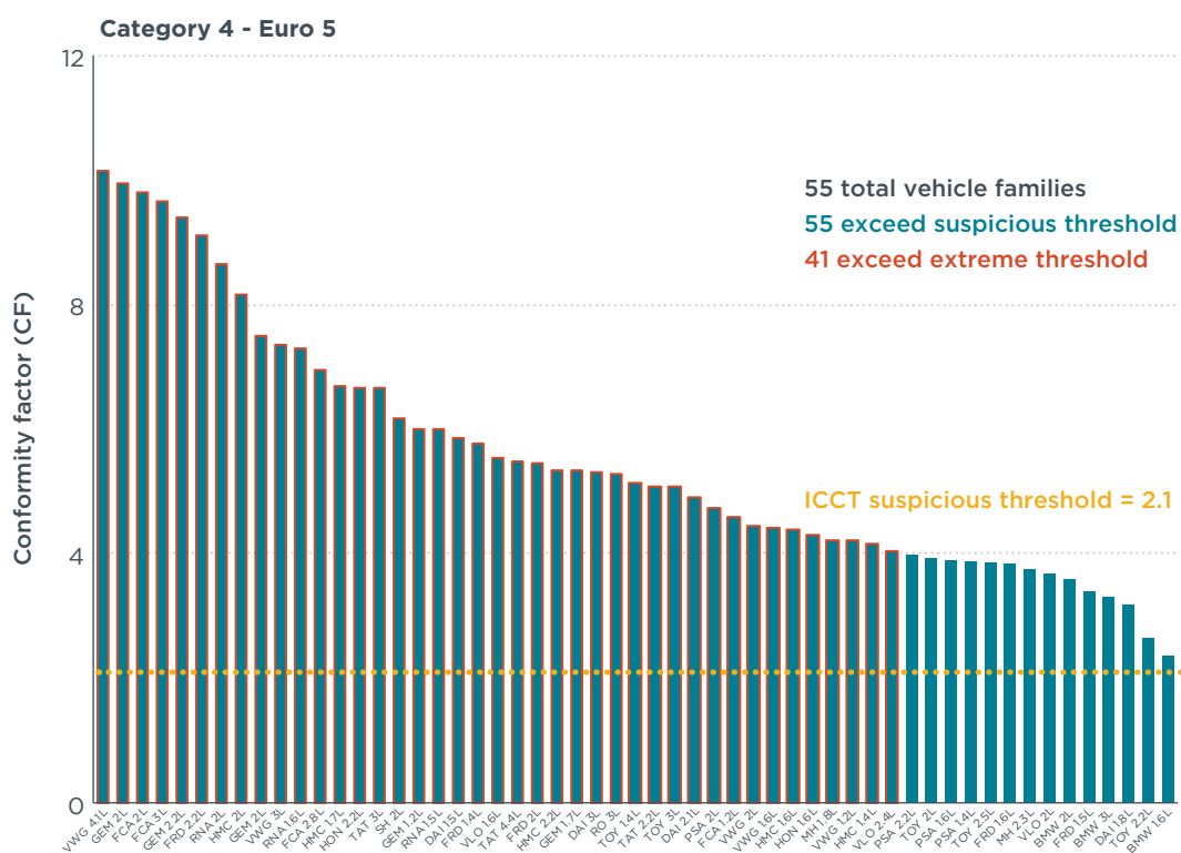
Figure 14. Average NO x conformity factors from Category 4 remote sensing by Euro 5 diesel cars, grouped by vehicle engine family. The red outline indicates that the engine family's average emissions exceed the extreme threshold (CF = 4.0).
