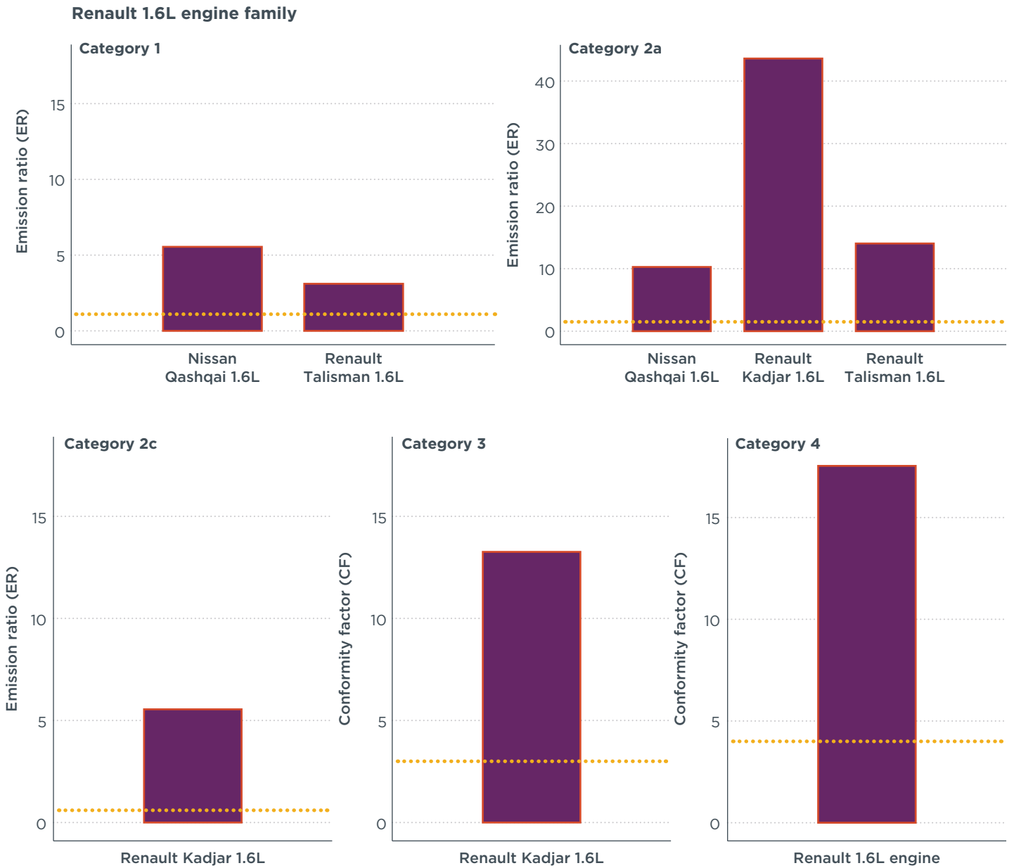
Figure D1. Tests results by vehicle model for one vehicle engine family (Renault 1.6L Euro 6 engine). The yellow dotted lines show the suspicious thresholds. Nearly all tests exceed the extreme threshold of their respective categories.
