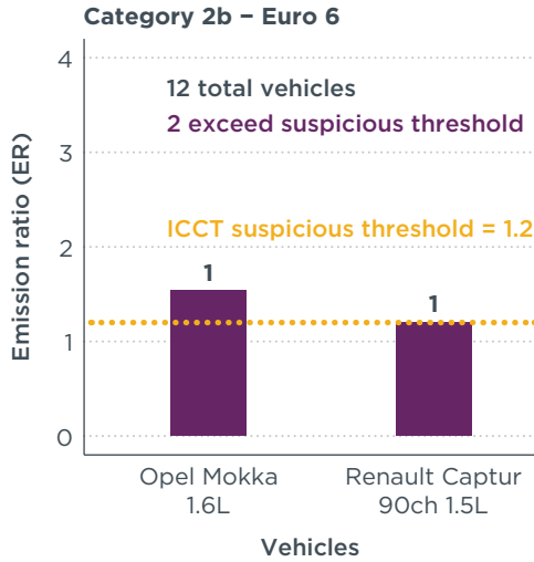
Figure 9. Average NO x emission ratios for Category 2b tests by diesel Euro 5 and 6 vehicle model, showing only those with tests exceeding the suspicious threshold. The count above each bar shows the number of tests performed.
