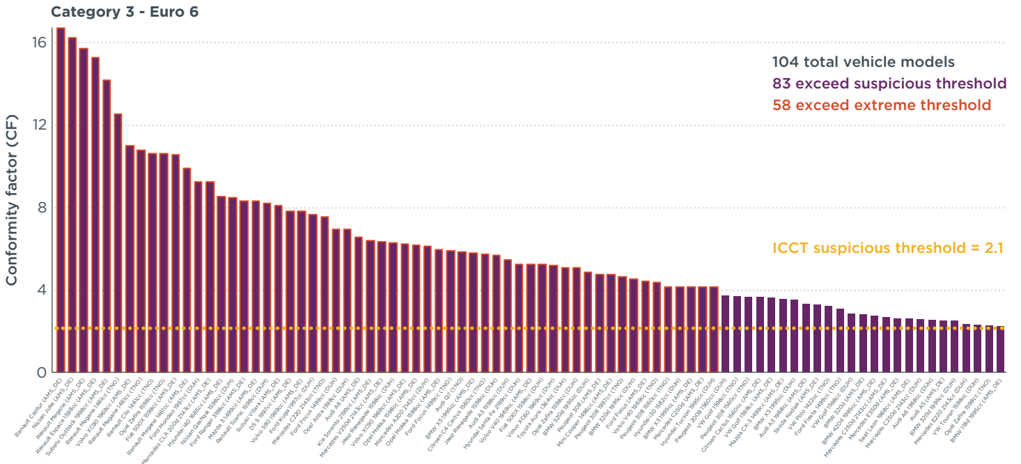
Figure 13. Average NO x conformity factors for independent Category 3 tests by Euro 6 diesel vehicle model, showing only those with averages exceeding the suspicious threshold. The test source is indicated in parenthesis. The red outline indicates that the vehicle model's average emissions exceed the extreme threshold (CF = 4.0).
