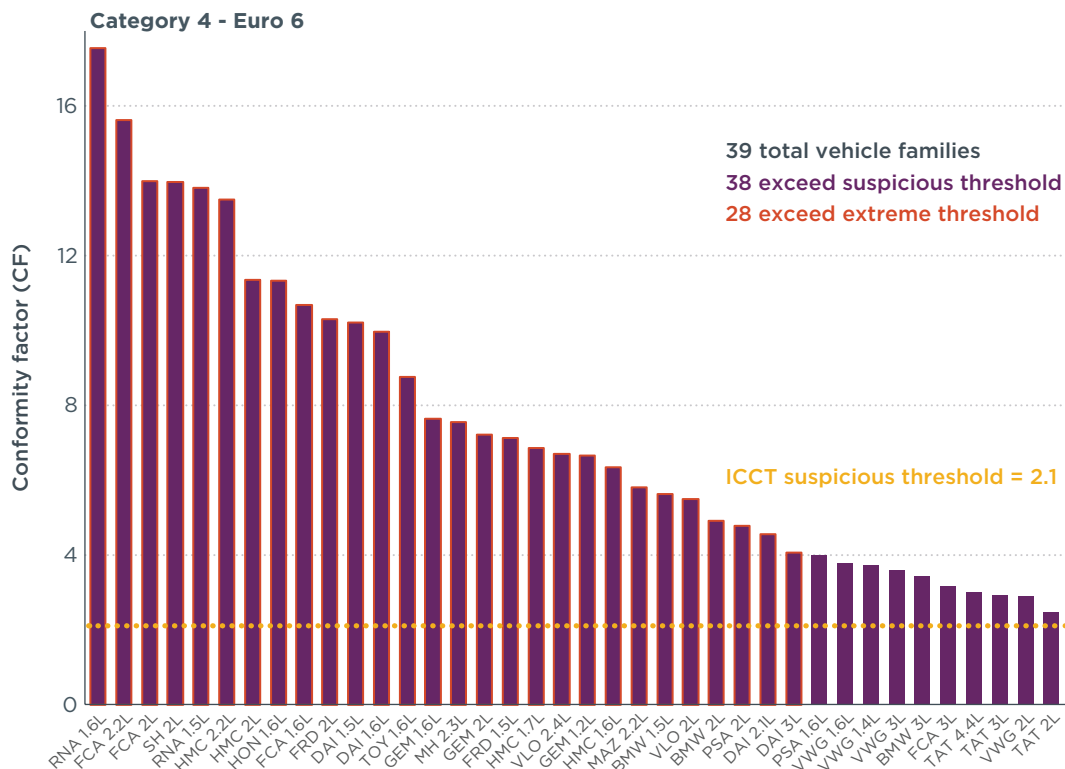
Figure 15. Average NO x conformity factors from Category 4 remote sensing by Euro 6 diesel cars, grouped by vehicle engine family, showing only those with averages exceeding the suspicious thresholds. The red outline indicates that the engine family's average emissions exceed the extreme threshold (CF = 4.0).
