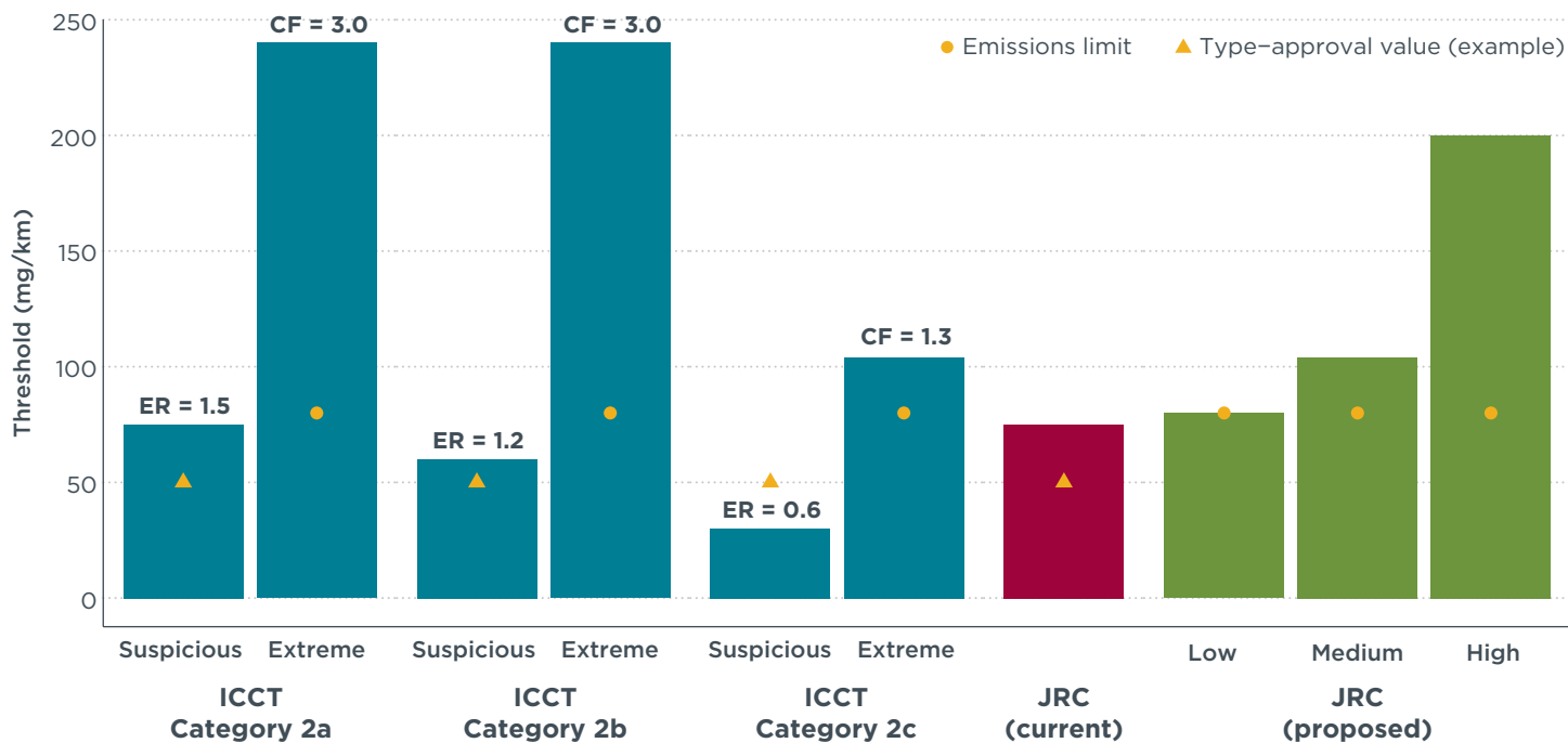
Figure 4. ICCT recommended thresholds compared to existing and proposed thresholds for Category 2 tests, using an example of a Euro 6 vehicle type-approved at 50 mg NO x /km.
