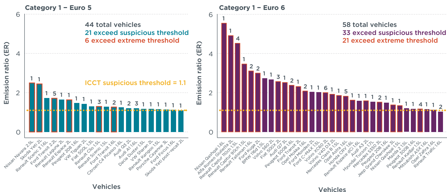
Figure 7. Average NO x emission ratios for Category 1 tests by diesel Euro 5 and 6 vehicle model, showing only those with tests exceeding the suspicious threshold. The count above each bar shows the number of tests performed and the red outline indicates that at least one test for the given vehicle model exceeds the extreme threshold (CF = 1.3).
